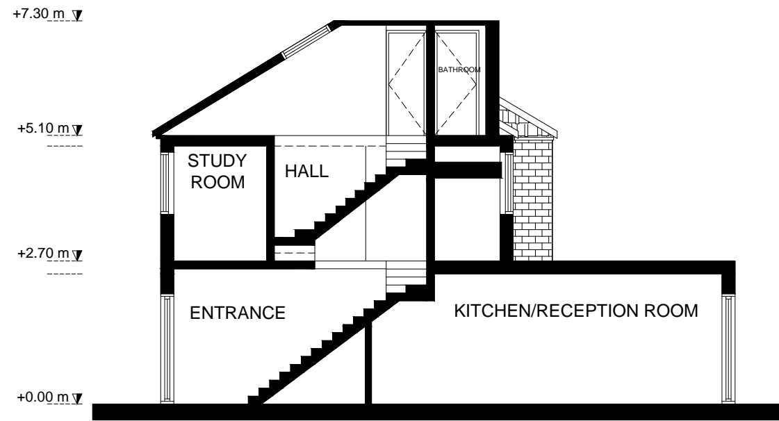
Proposed A-A Section
