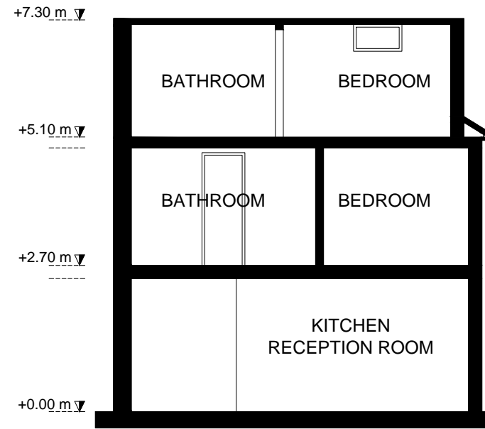
Existing B-B Section
