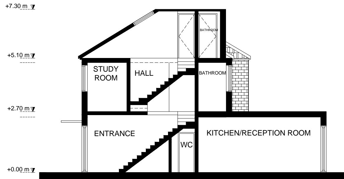
Existing A-A Section
