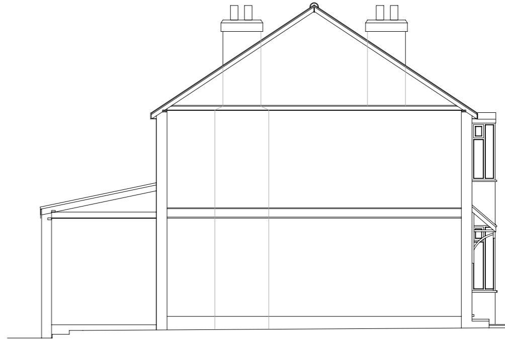
EXISTING SECTION 1:100
