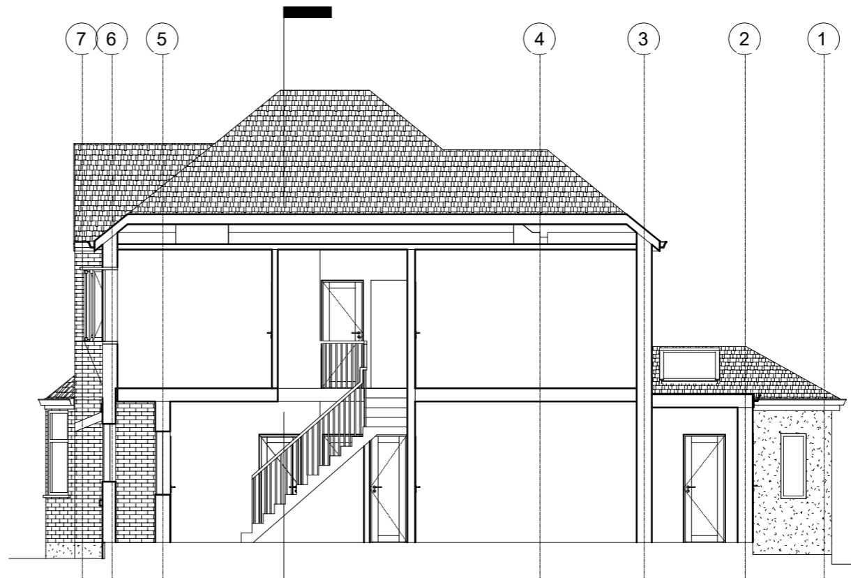
EXISTING SECTION
