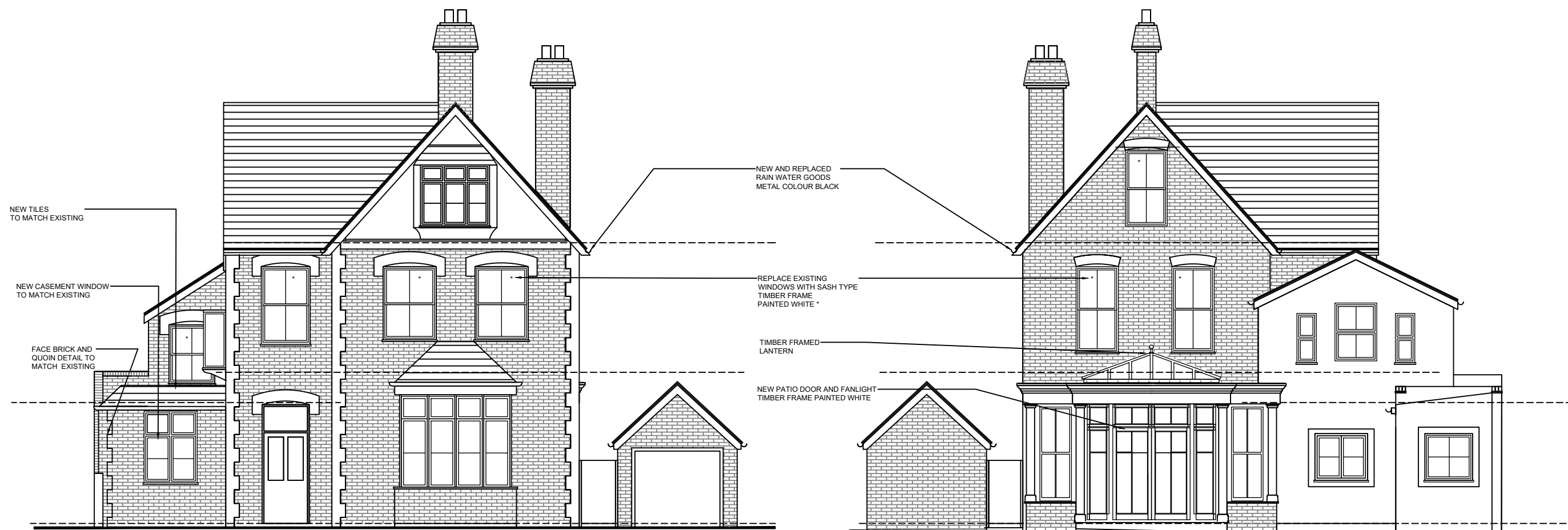
PLA PROPOSED NORTH EAST ELEVATION Scale 1:100
