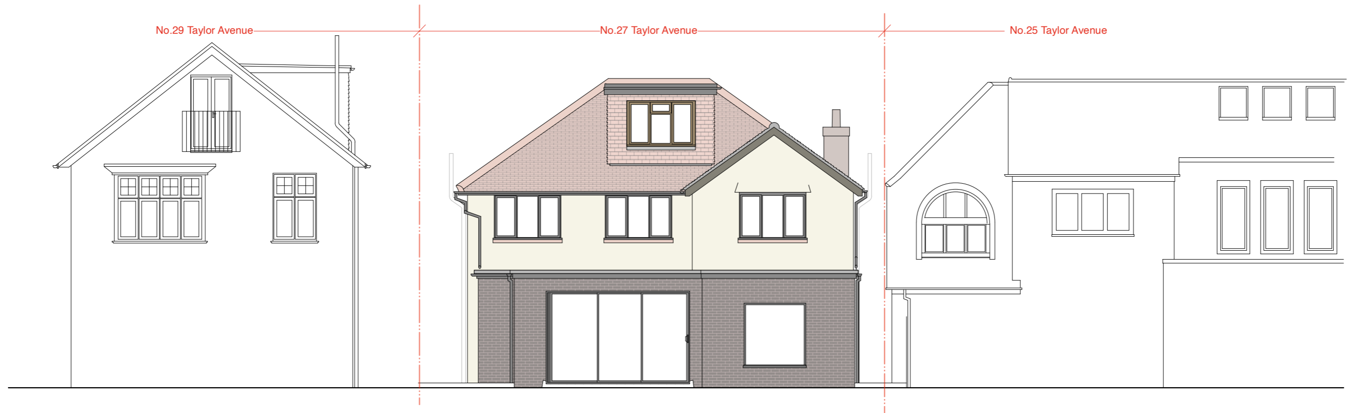
REAR ELEVATION EXISTING
