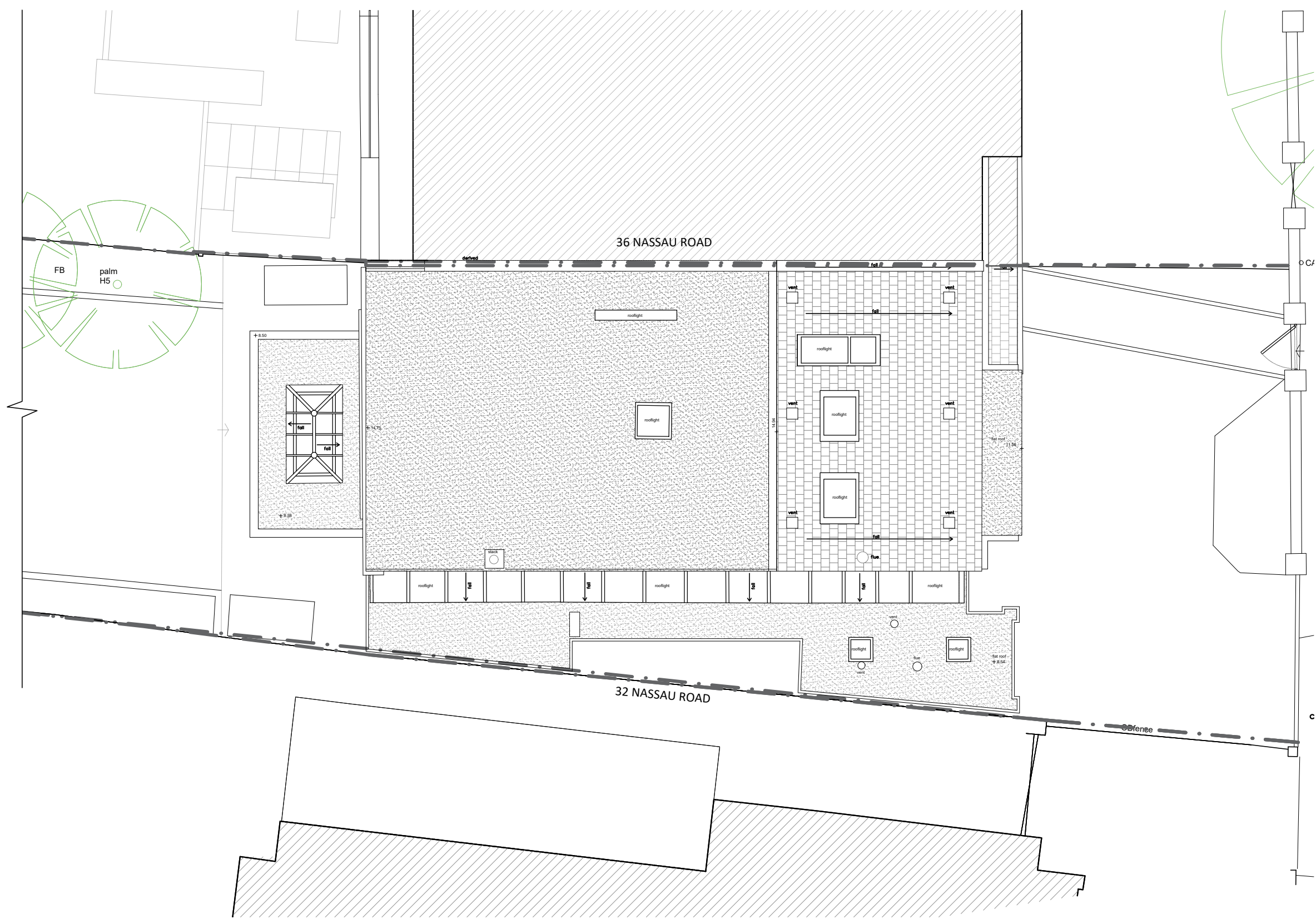
1 | ROOF PLAN AS EXISTING 00-13 | SCALE: 1:100 @ A3 // 1:50 @ A1
