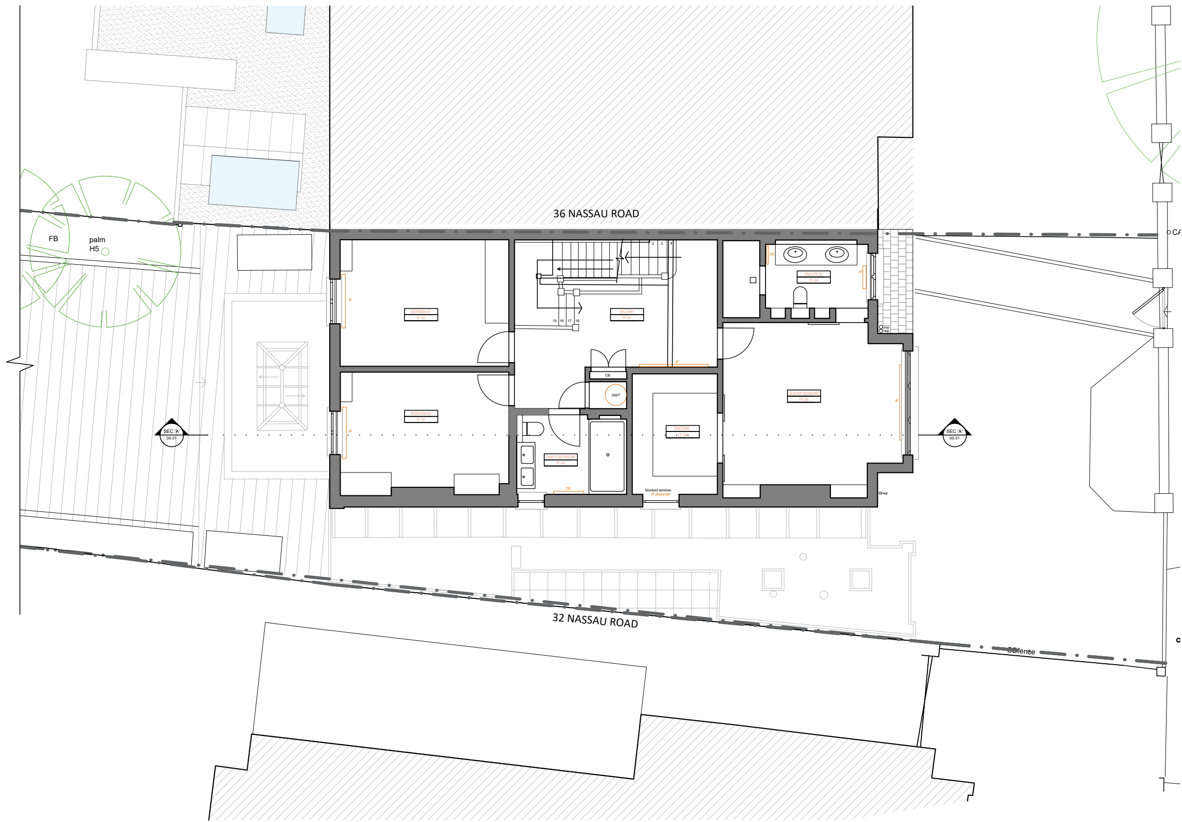
1 | FIRST FLOOR PLAN AS EXISTING 00-11 | SCALE: 1:100 @ A3 // 1:50 @ A1
