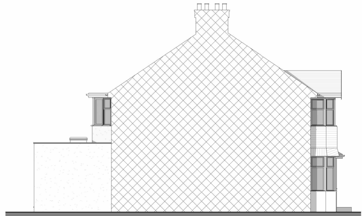
Side 2 Elevation
