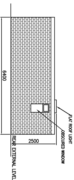
PROPOSED BACK ELEVATION
