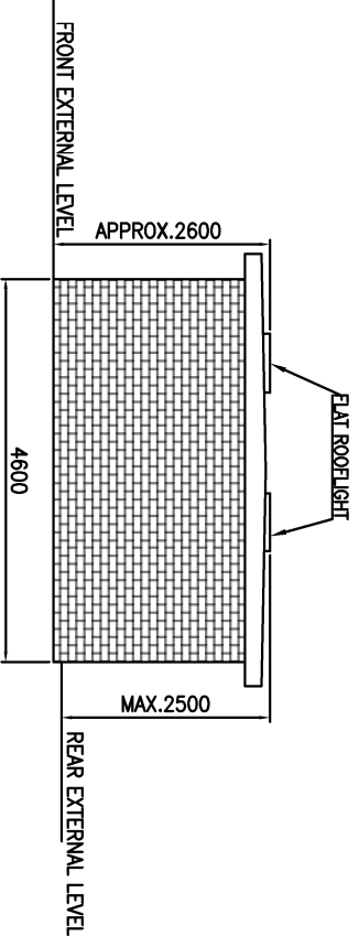
PROPOSED SIDE ELEVATION B-B
