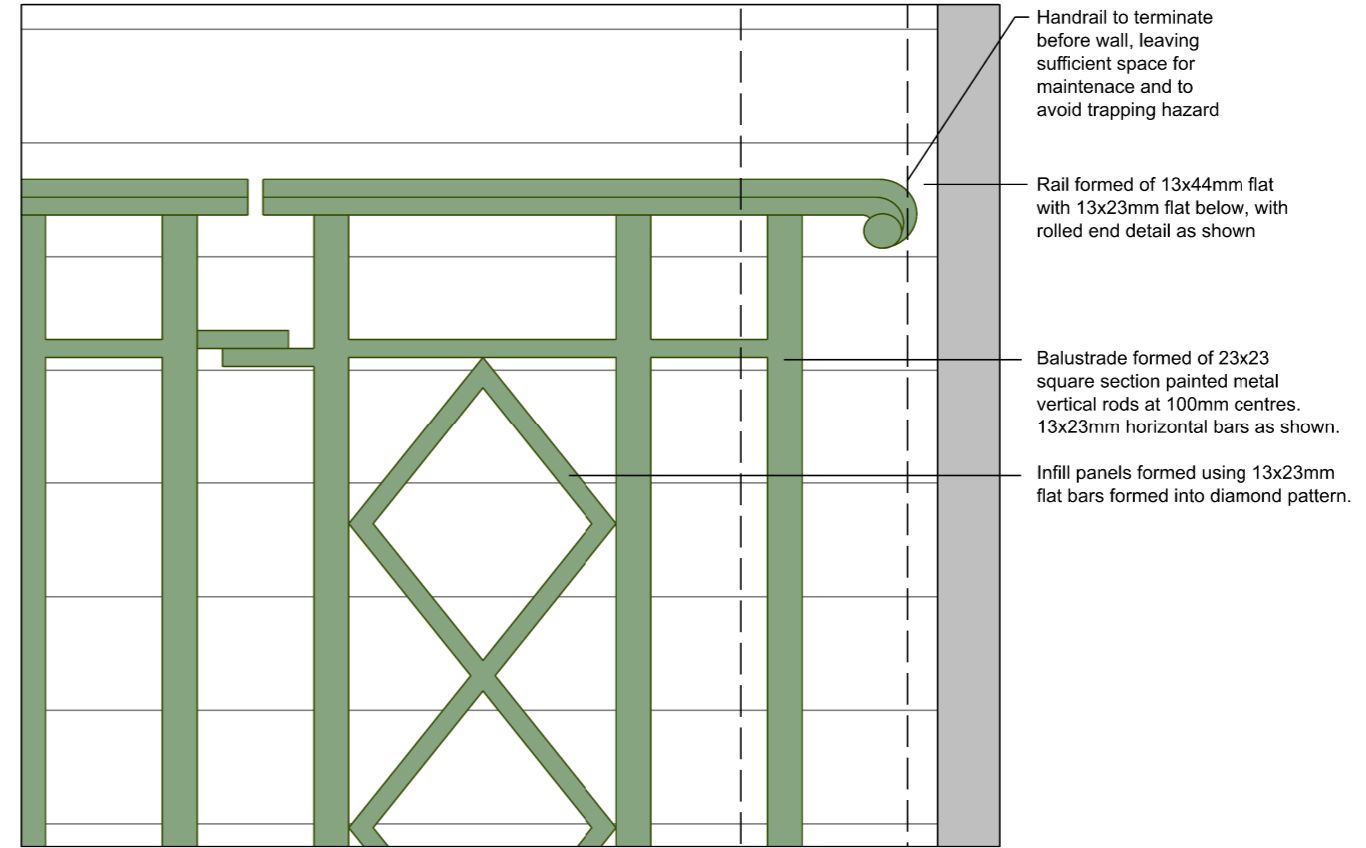
Detail of proposed handrail & guarding 1:5 @ A3
