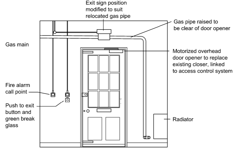
Elevation 3. Internal Elevation
