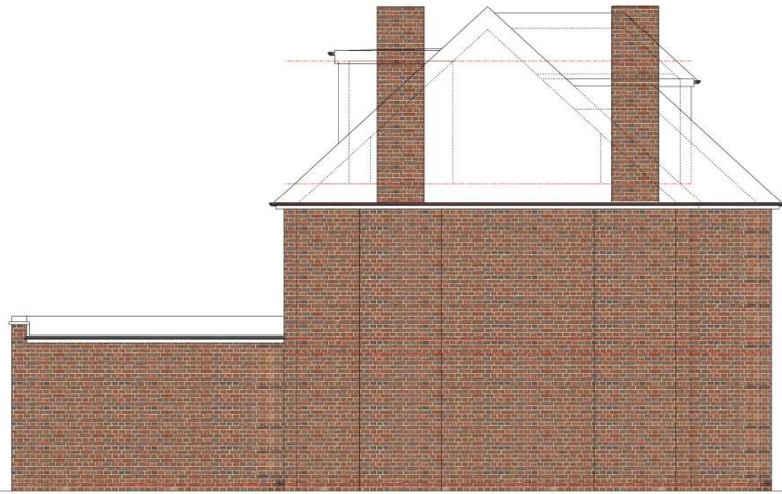
EXTG SOUTH ELEVATION 1:100 @A3
