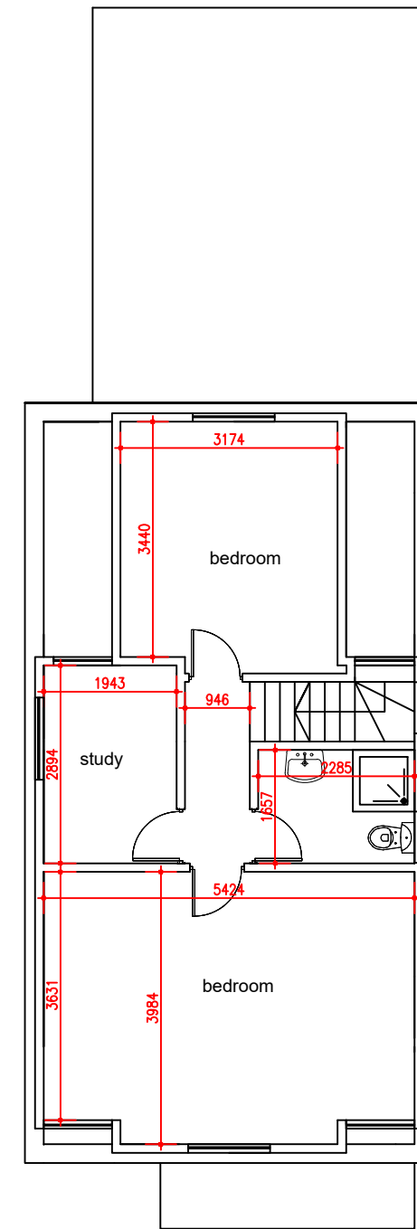
PROPOSED LOFT FLOOR PLAN
