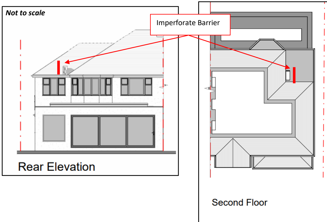
Figure 6.1 Proposed approximate location of imperforate barrier
