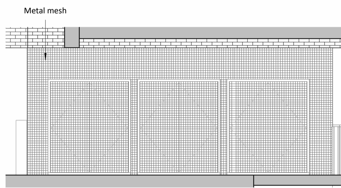
North Elevation 1 : 50
