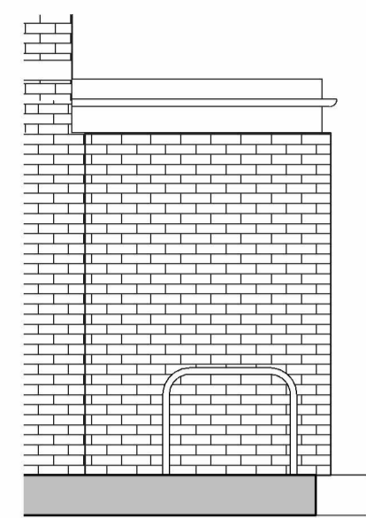
South Elevation 1 : 50
