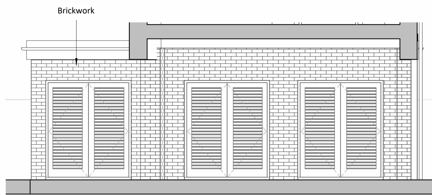
West Elevation 1 : 50
