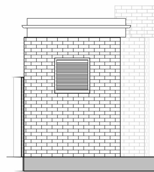
North Elevation 1 : 50
