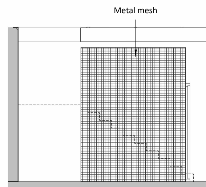
West Elevation 1 : 50
