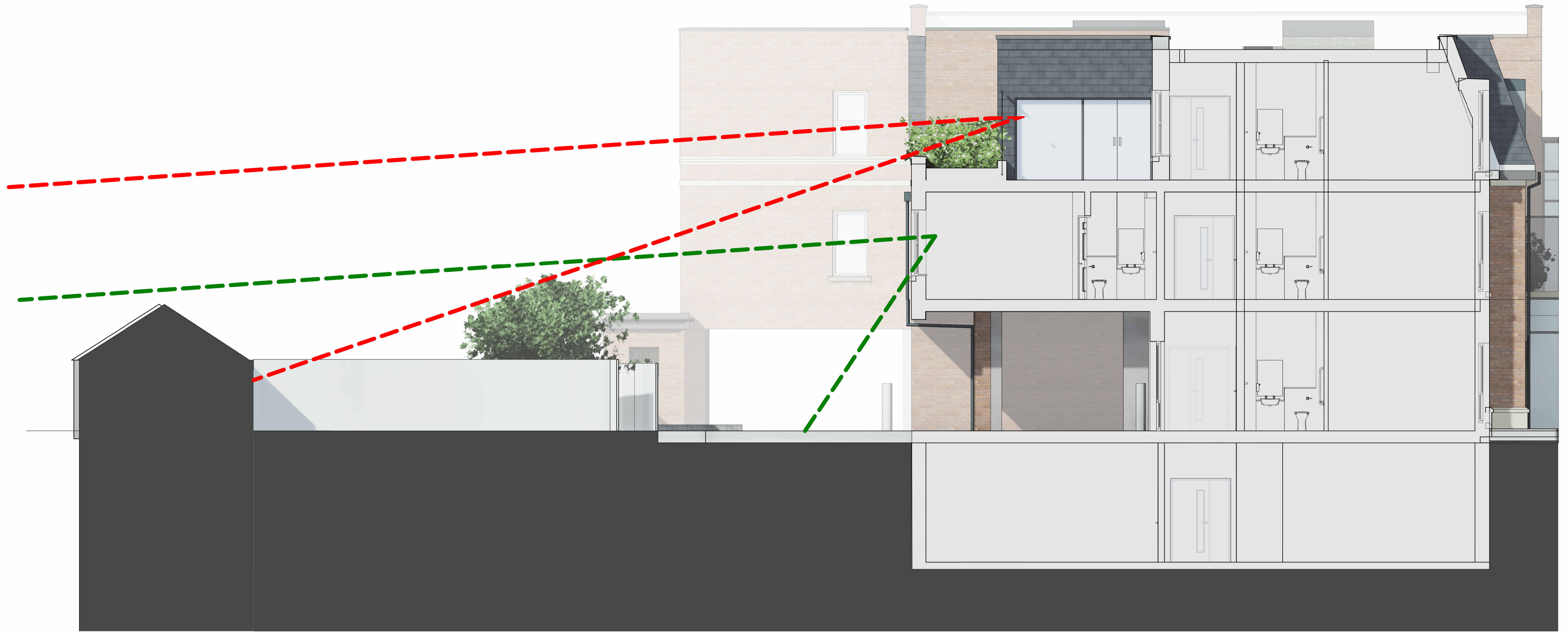
PROPOSED DETAILED SECTION A1 1 : 50
