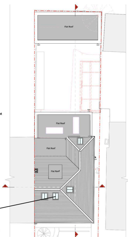
Roof Plan
