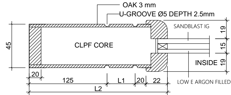
A CROSS SECTION SCALE 1 : 3
