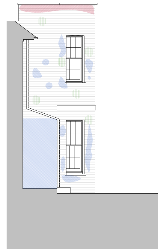
Existing East Elevation JJ scale 1:100
