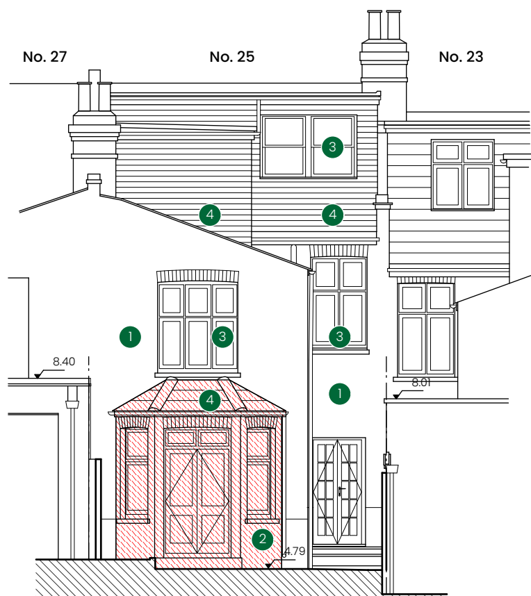
Existing elevation
