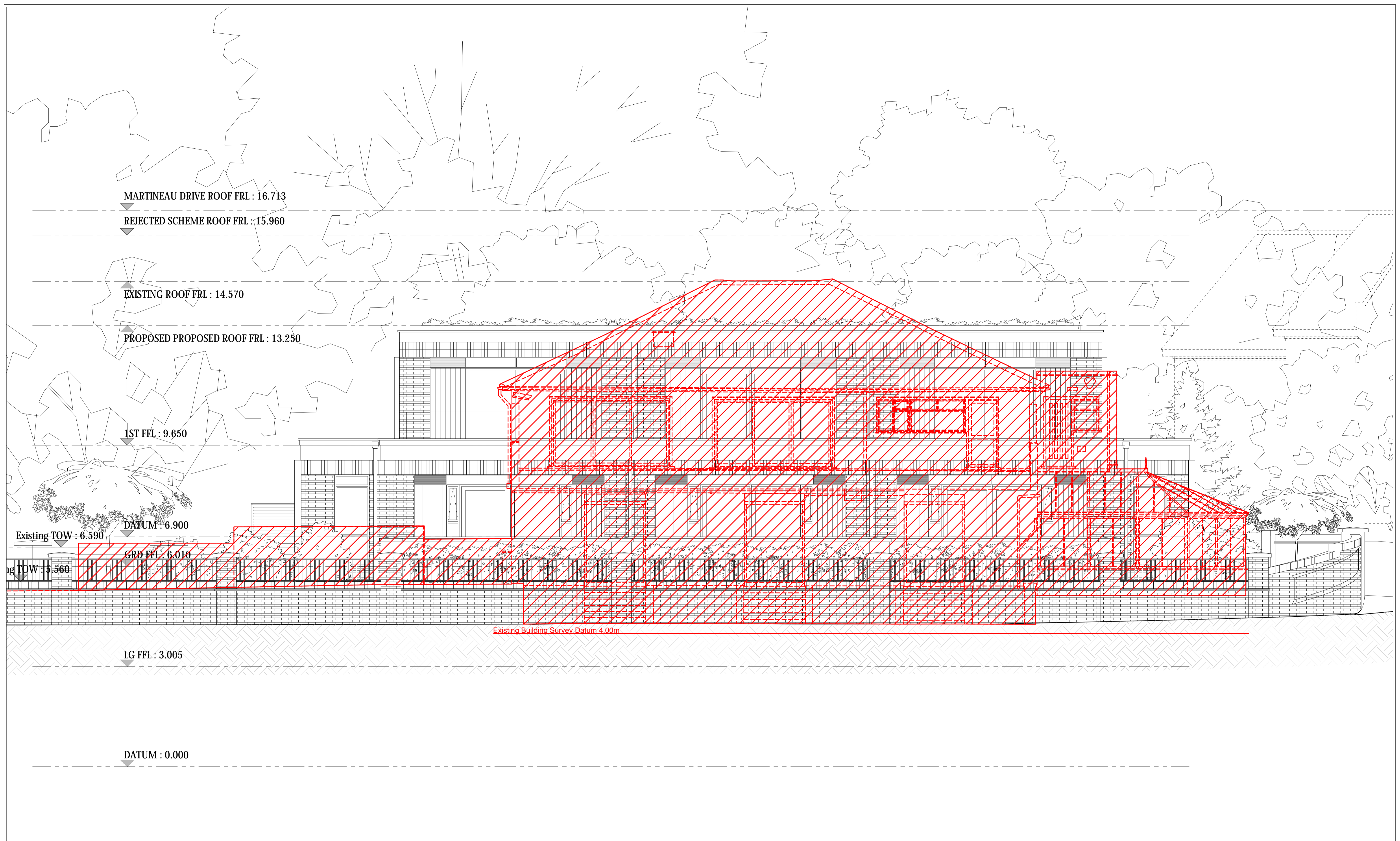
Proposed North Elevation and Existing Elevation Dotted Scale @ 1:50
