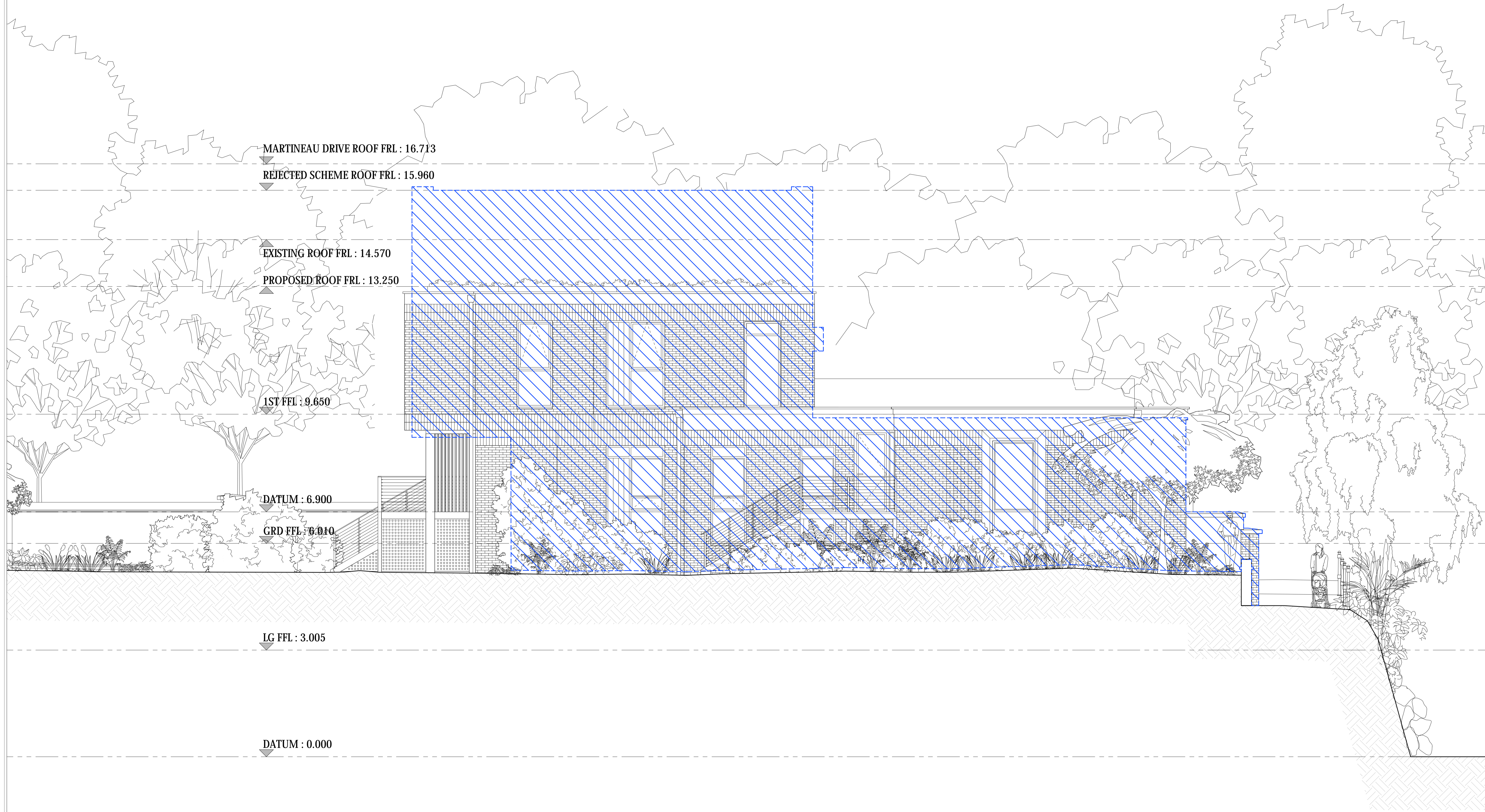
Proposed East Elevation and Existing Elevation Dotted Scale @ 1:50
