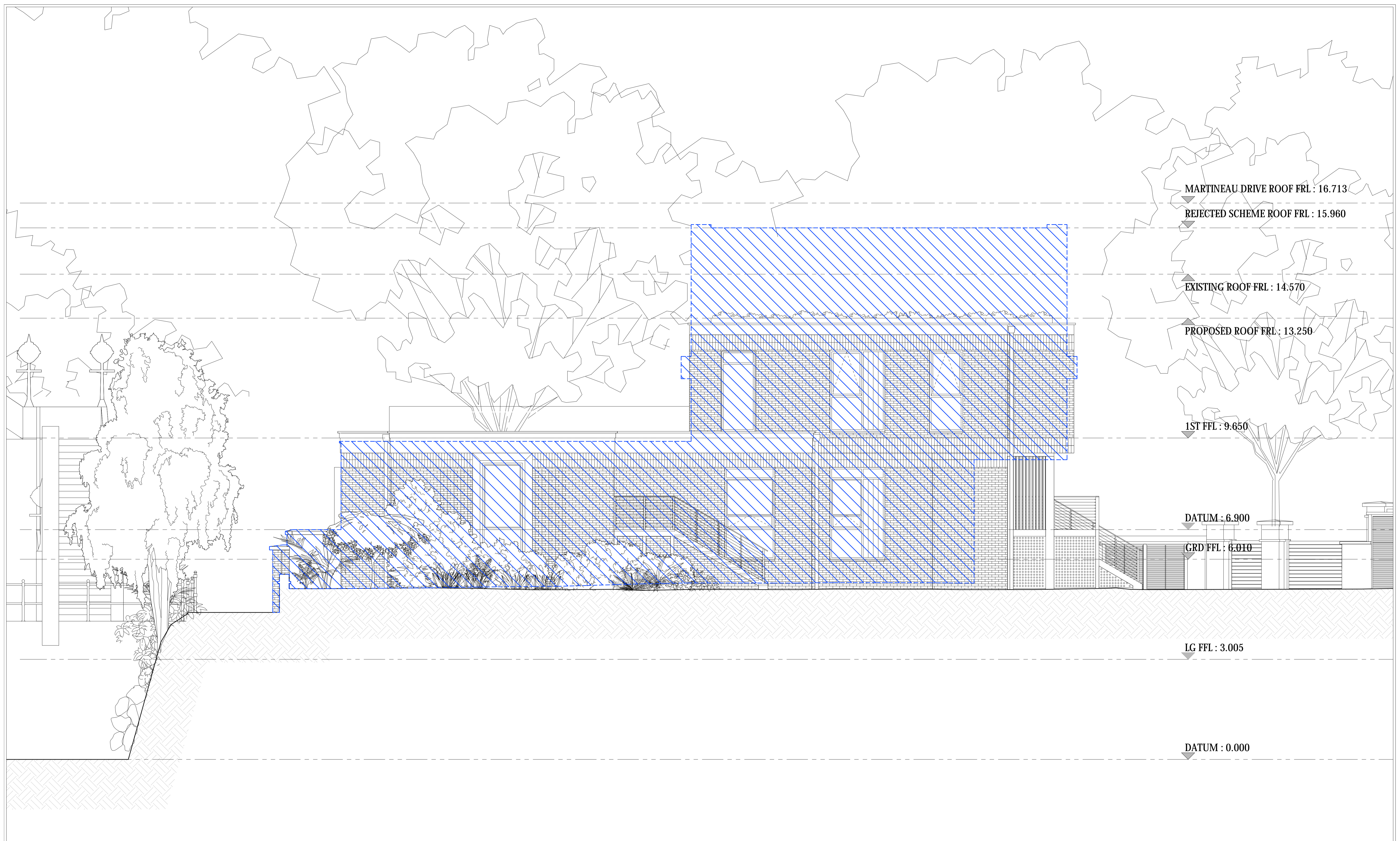
Proposed West Elevation and Rejected Scheme Dotted Scale @ 1:50
