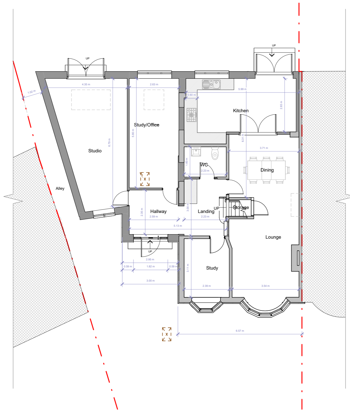
Ground Floor
