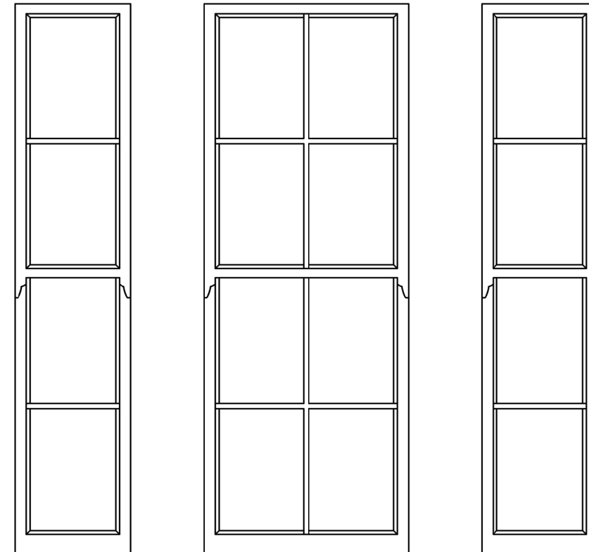
W2 Proposed Sash Replacement 1:20 @ A3
