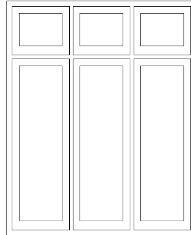
W4 Proposed Reglazing only 1:20 @ A3
