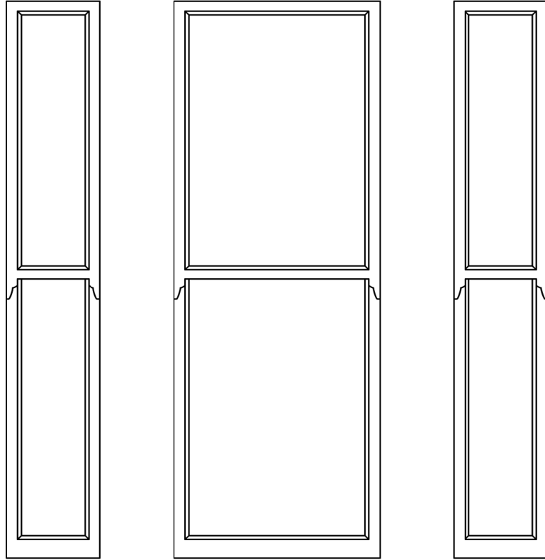
W3 Proposed Sash replacement 1:20 @ A3
