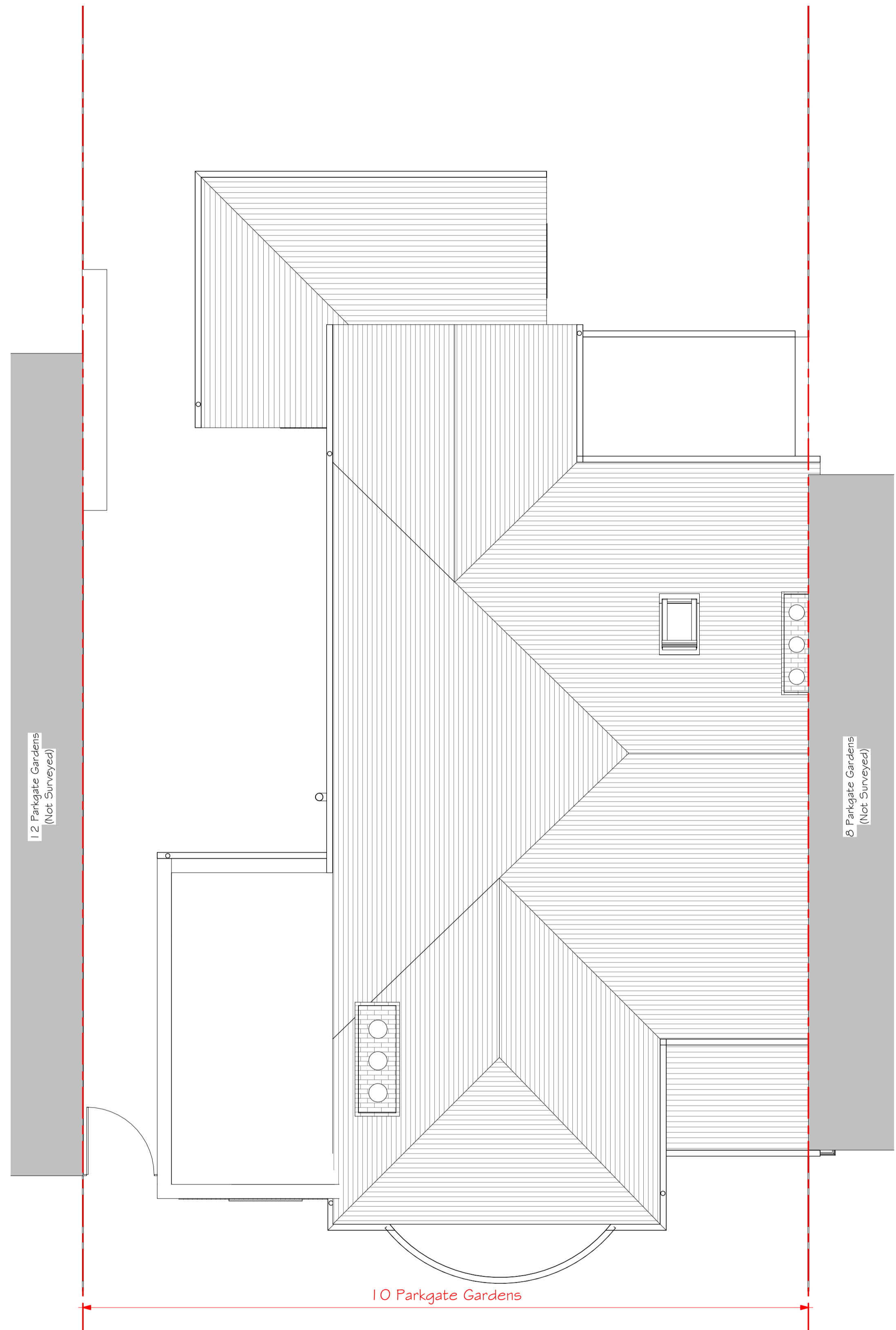
1 Existing Roof Plan 1 : 50
