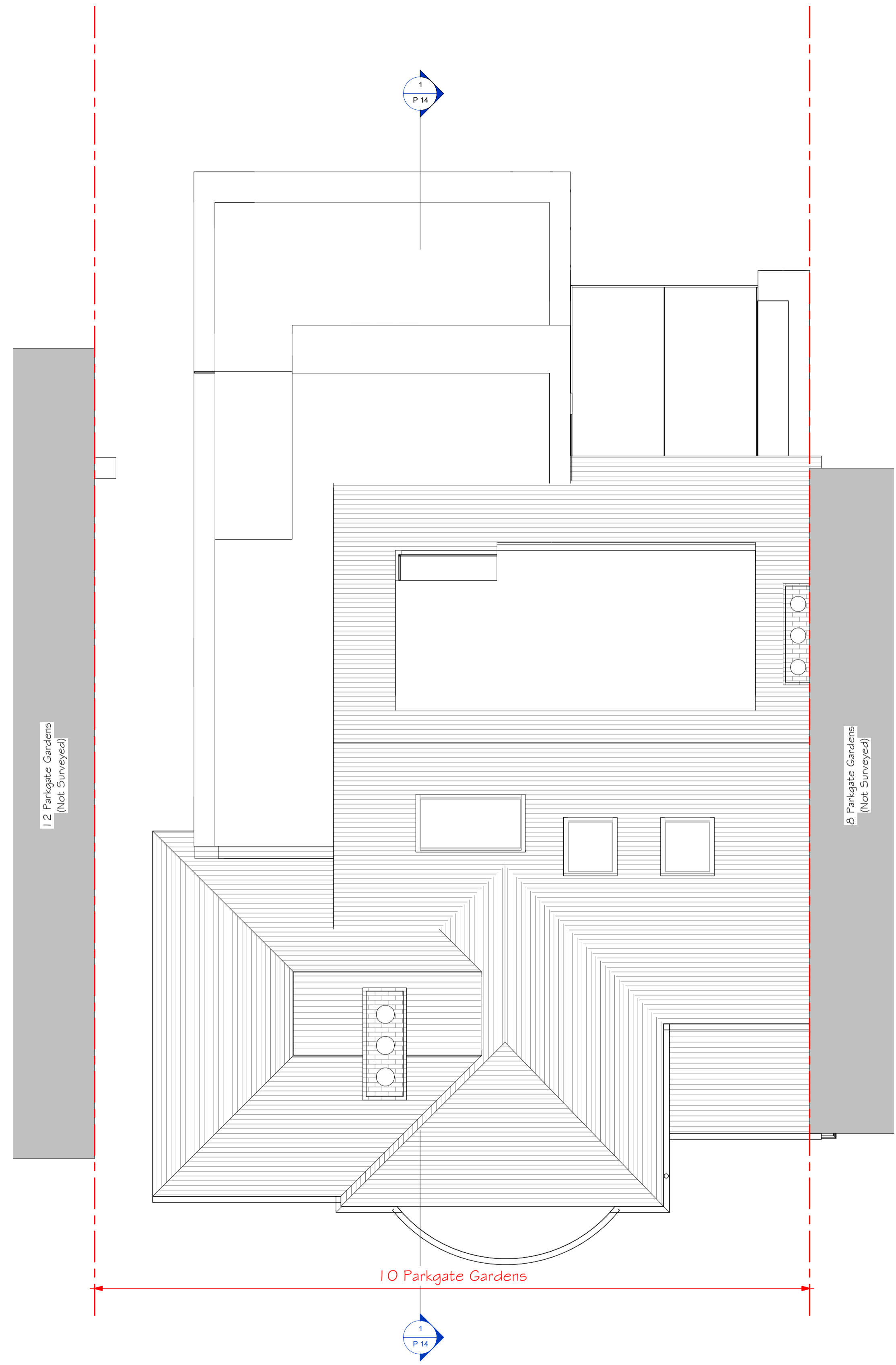
1 Proposed Roof Plan 1 : 50
