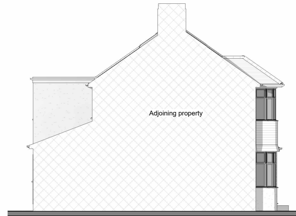
Side 2 Elevation
