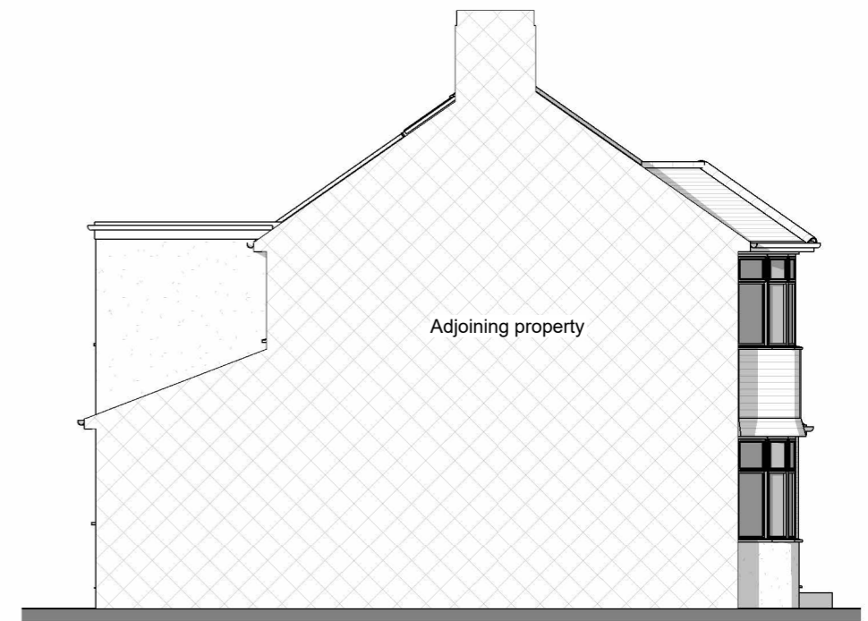
Side 2 Elevation
