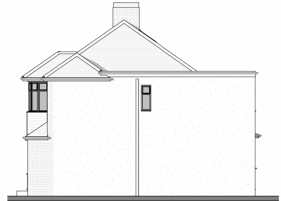
Side 1 Elevation
