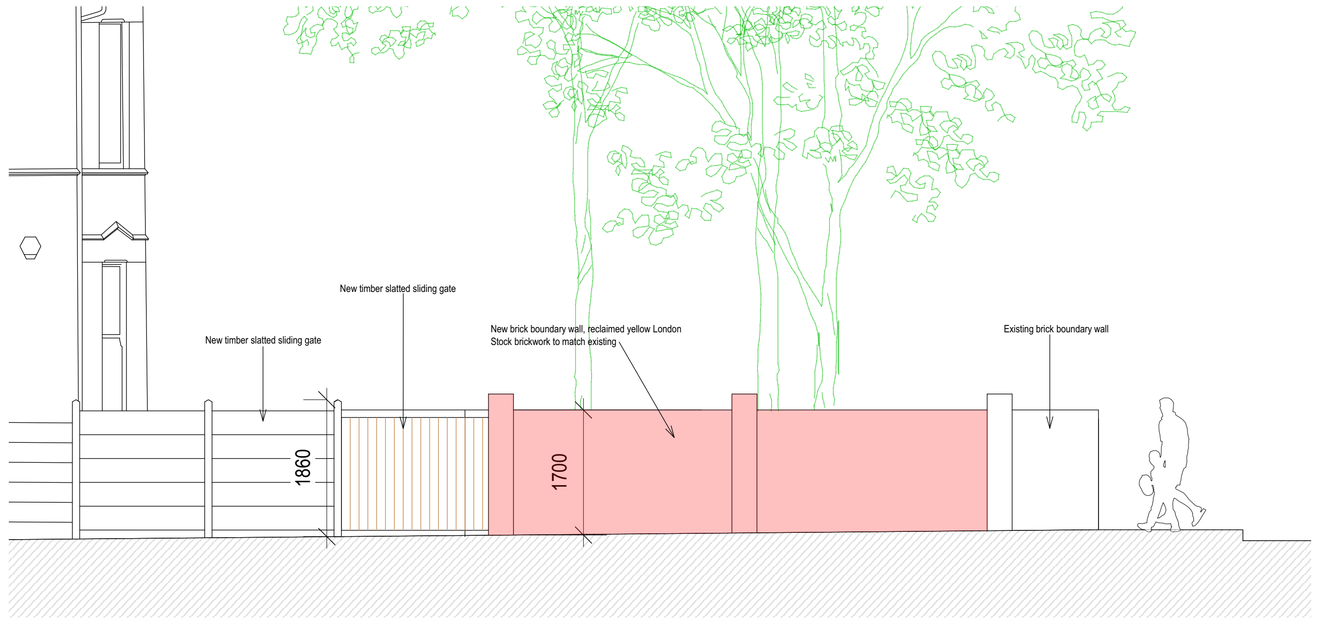
1 DETAILED ELEVATION OF PROPOSED BOUNDARY WALL AT REFUSE STORE 1:50
