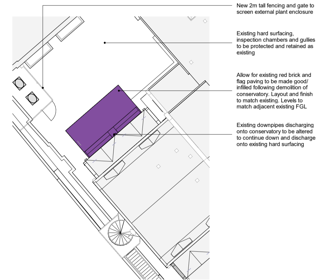
5 Planning - Proposed Hard Landscaping - Main Building 01 1 : 200
