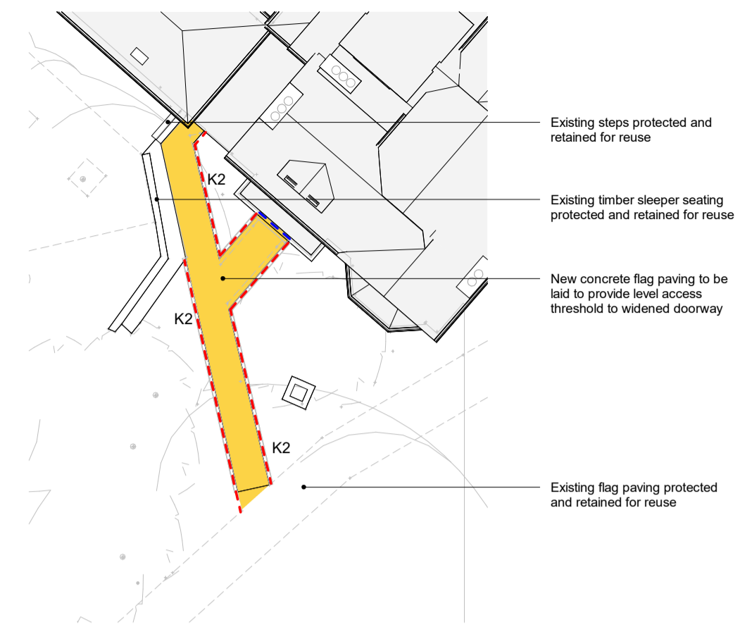
3 Planning - Proposed Hard Landscaping - Red House 1 : 200
