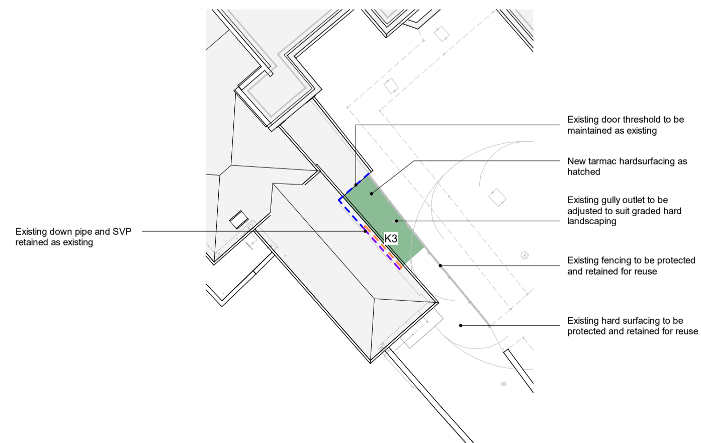
6 Planning - Proposed Hard Landscaping - Main Building 02 1 : 200
