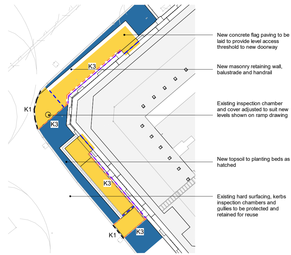
2 Planning - Proposed Hard Landscaping - SCTL 1 : 200
