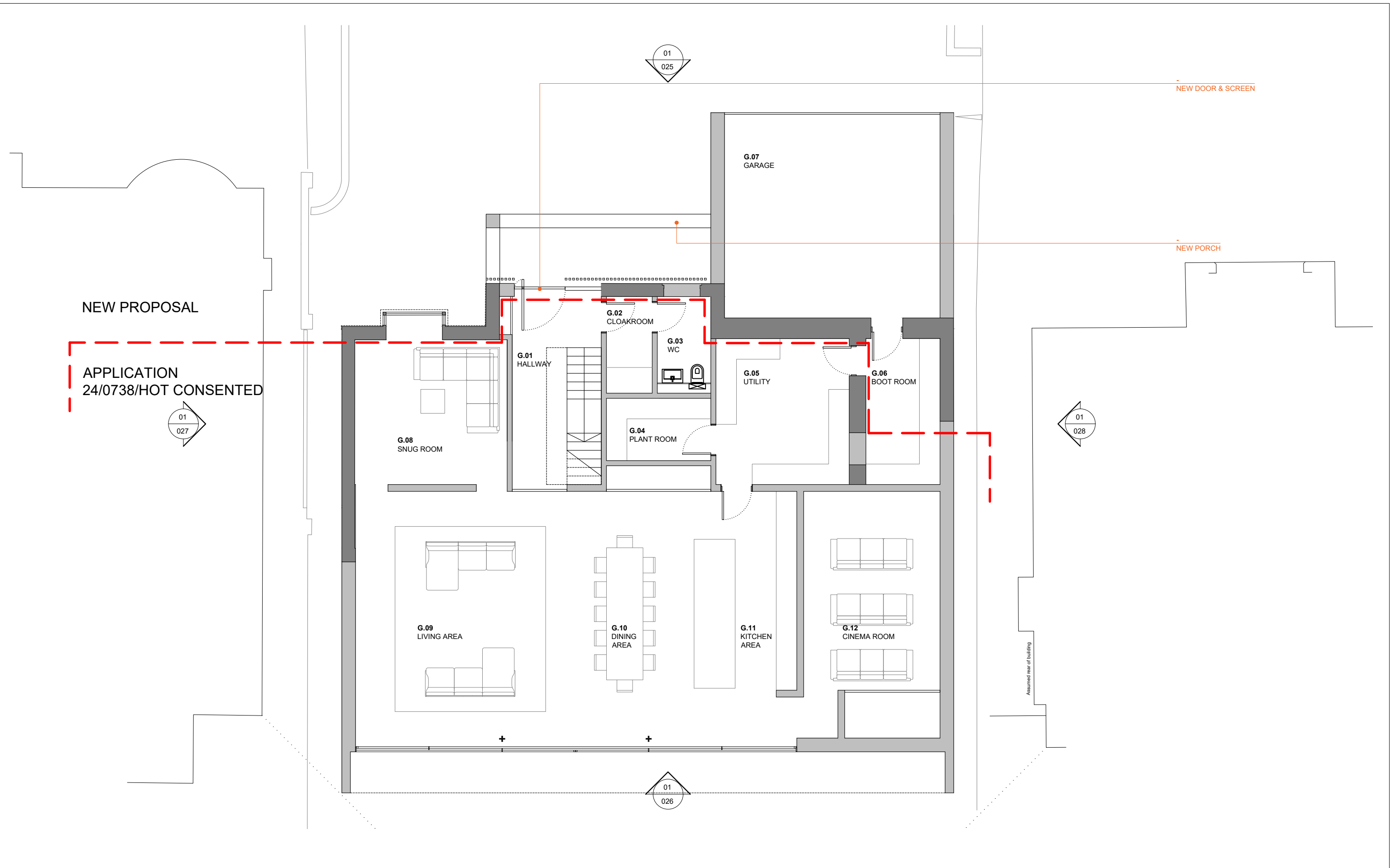
01 PROPOSED GROUND FLOOR PLAN 1:100 @A3
