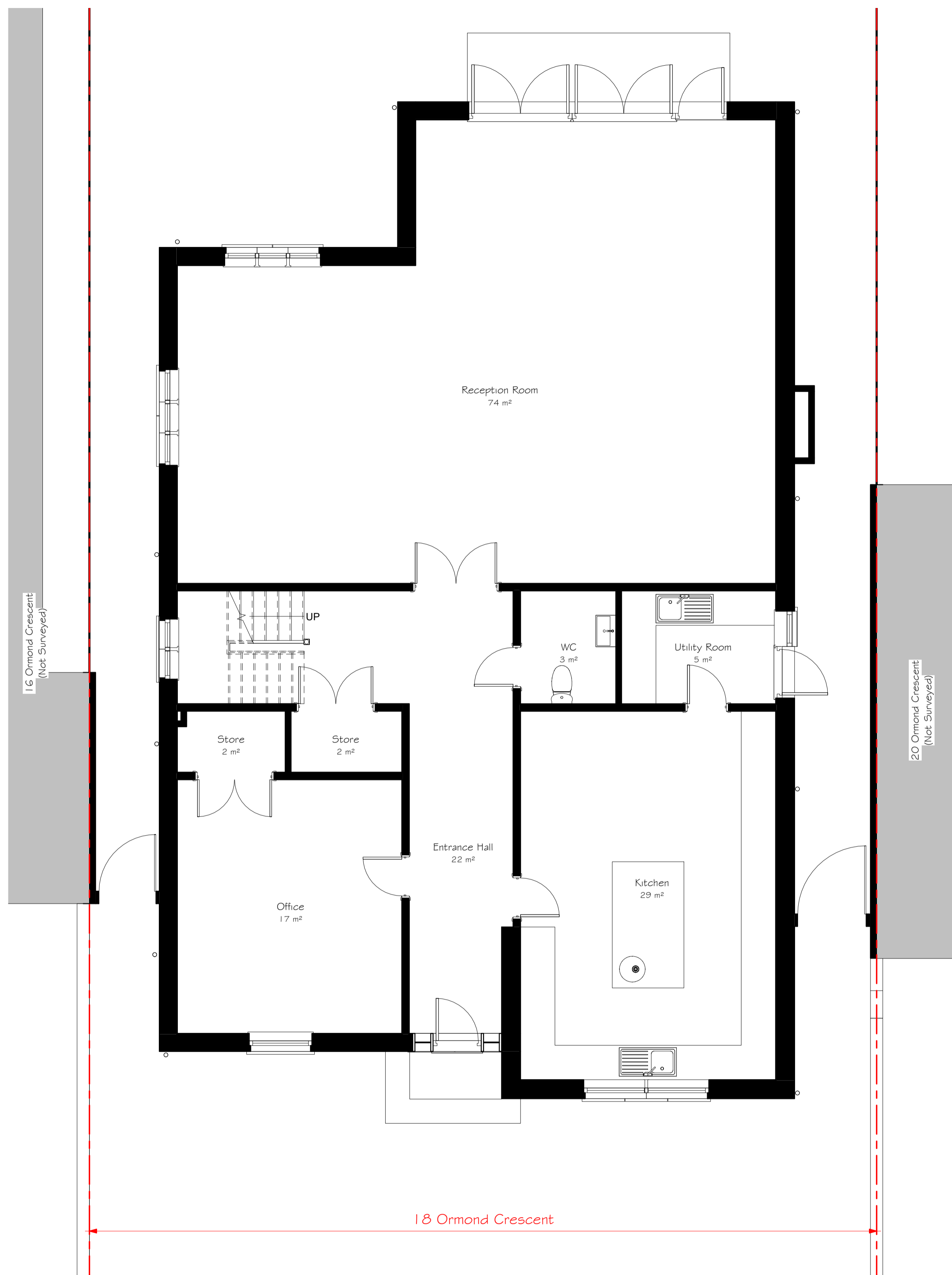
1 Existing Ground Floor 1 : 50
