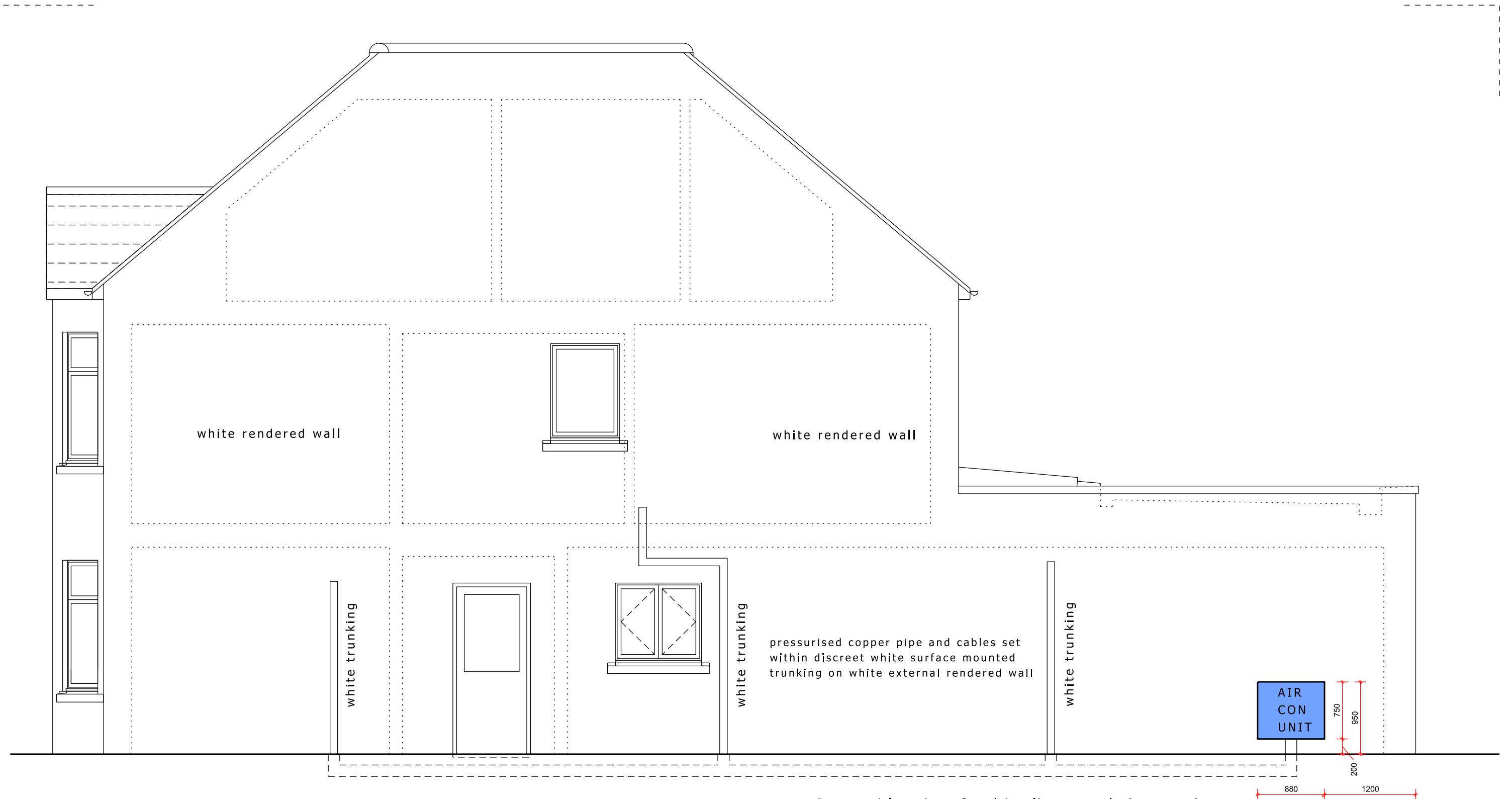
Proposed location of multi-split external air con unit (Mitsubishi SCM71ZS-W 7.1KW QR SCM80ZS-W 8KW, approx. 0.88m W x 0.75m H x 0.4m D), on floor mounting (refer to Noise and Vibration report for further information)
