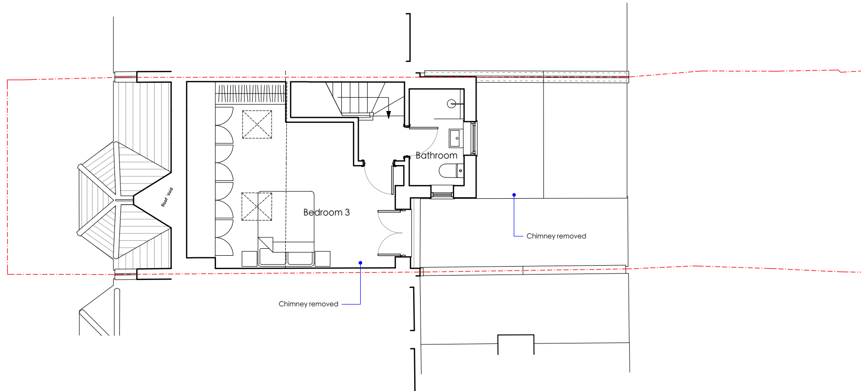
Second Floor Plan - As Proposed Scale 1:100 @ A3
