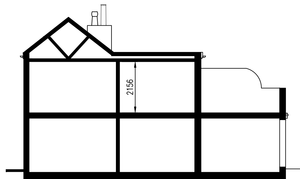
Existing Section 1:100
