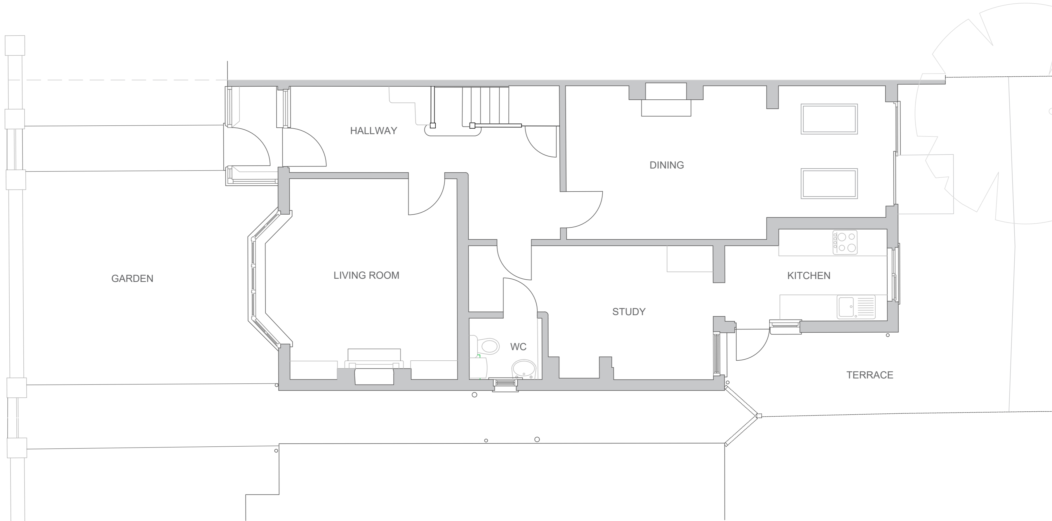
EXISTING GROUND FLOOR
