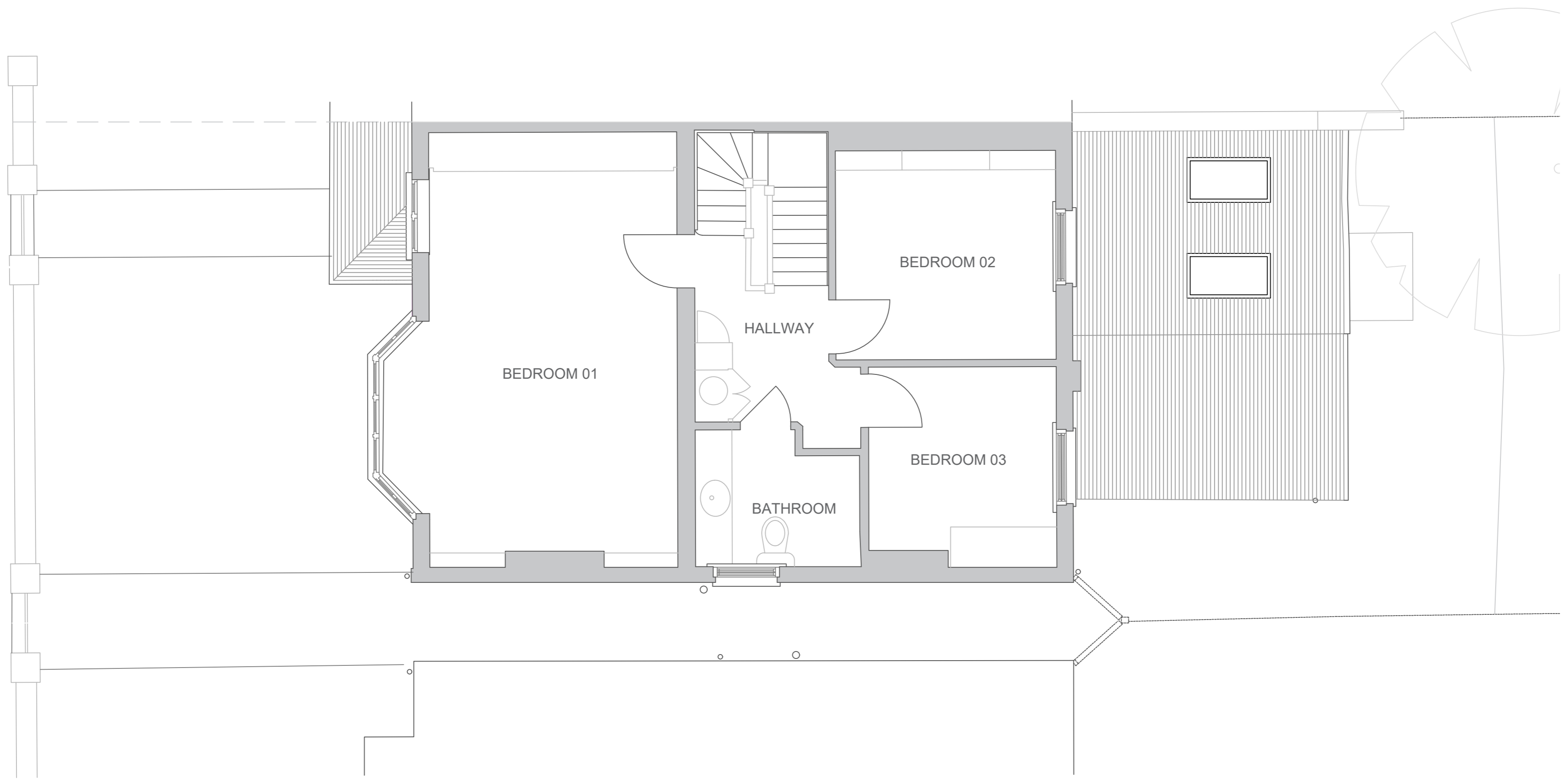
PROPOSED FIRST FLOOR
