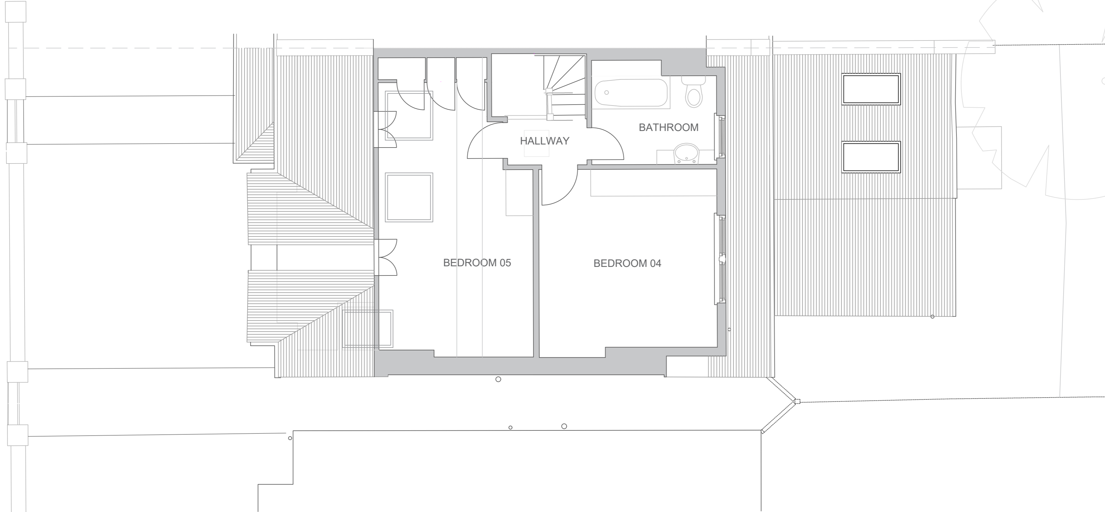
PROPOSED SECOND FLOOR
