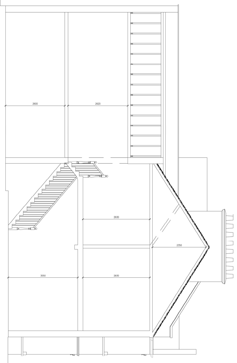
03 | EXISTING SECTION 1:100
