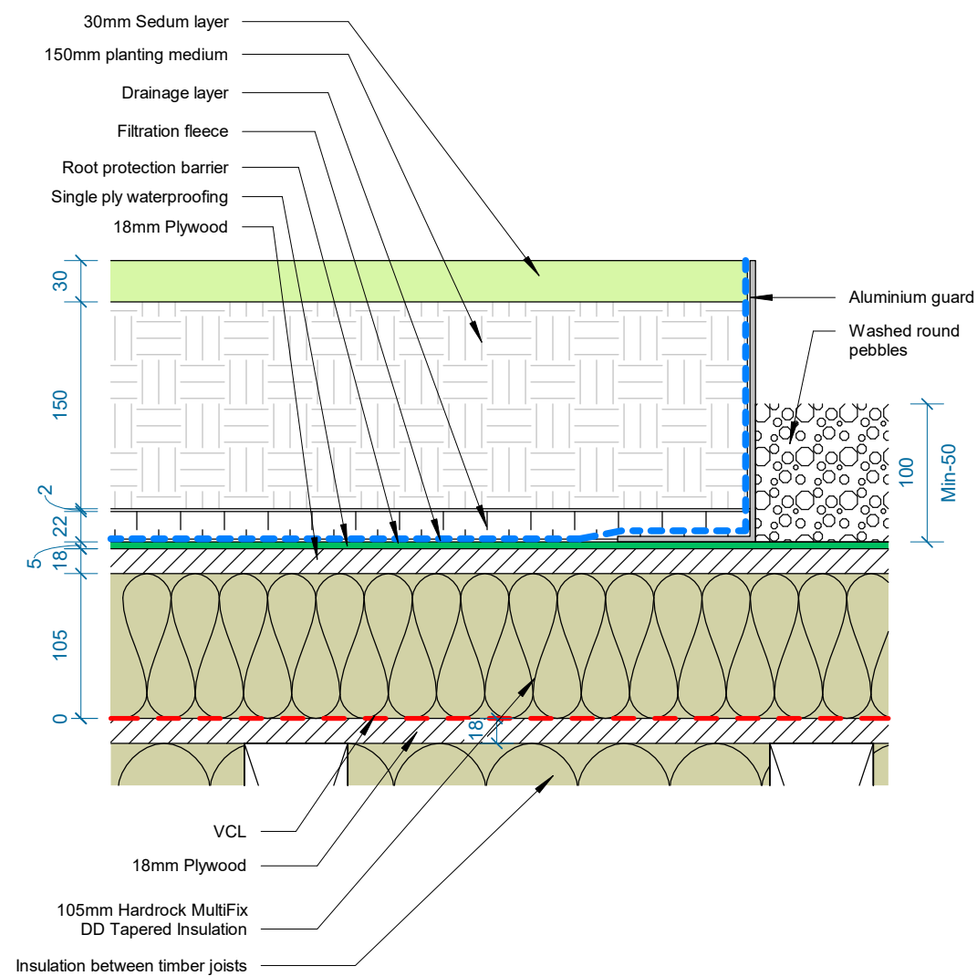
2 Intensive Green Roof Detail 1 : 5
