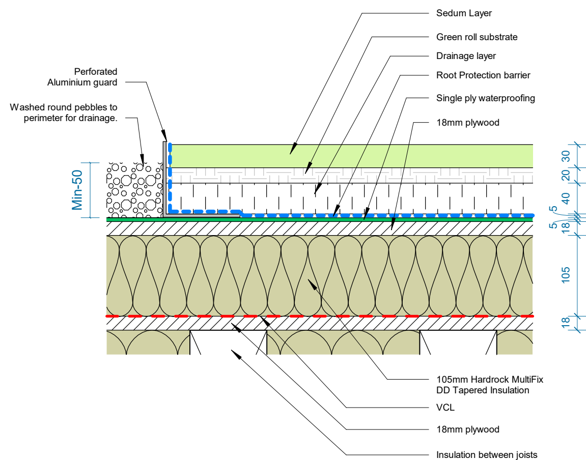
1 Extensive Green Roof Detail 1 : 5
