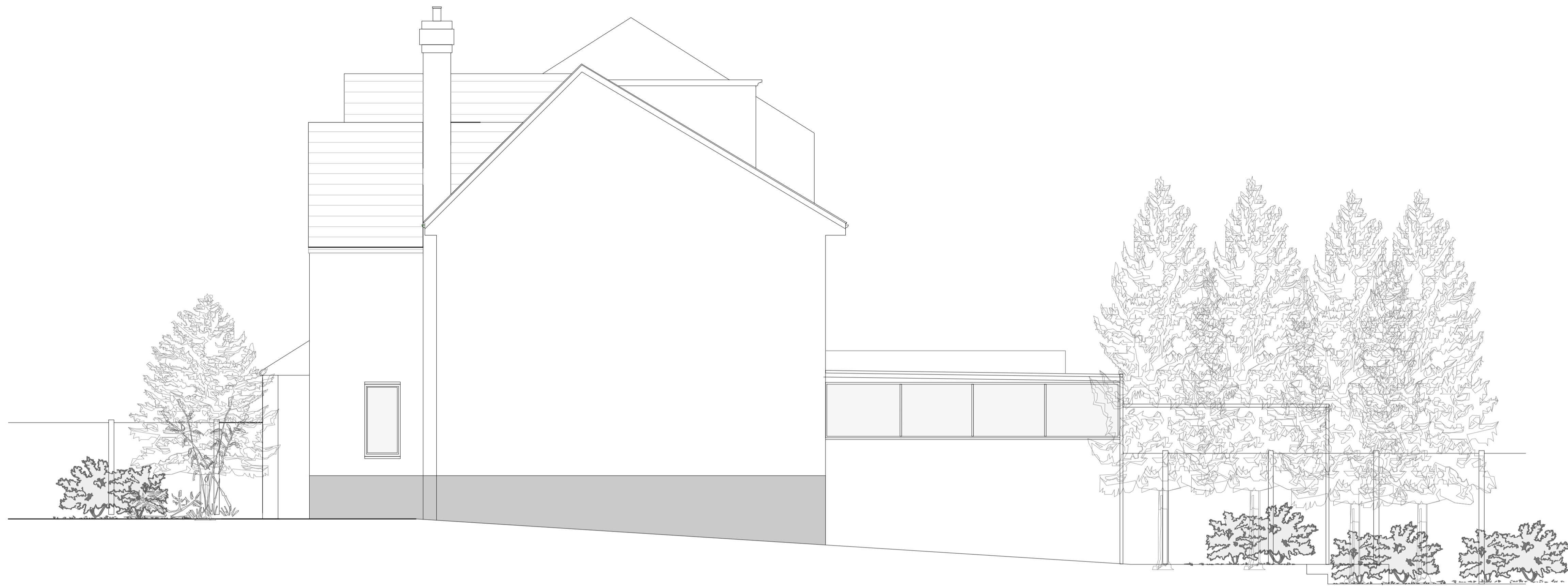
01 South Side Elevation - EXISTING scale 1:50
