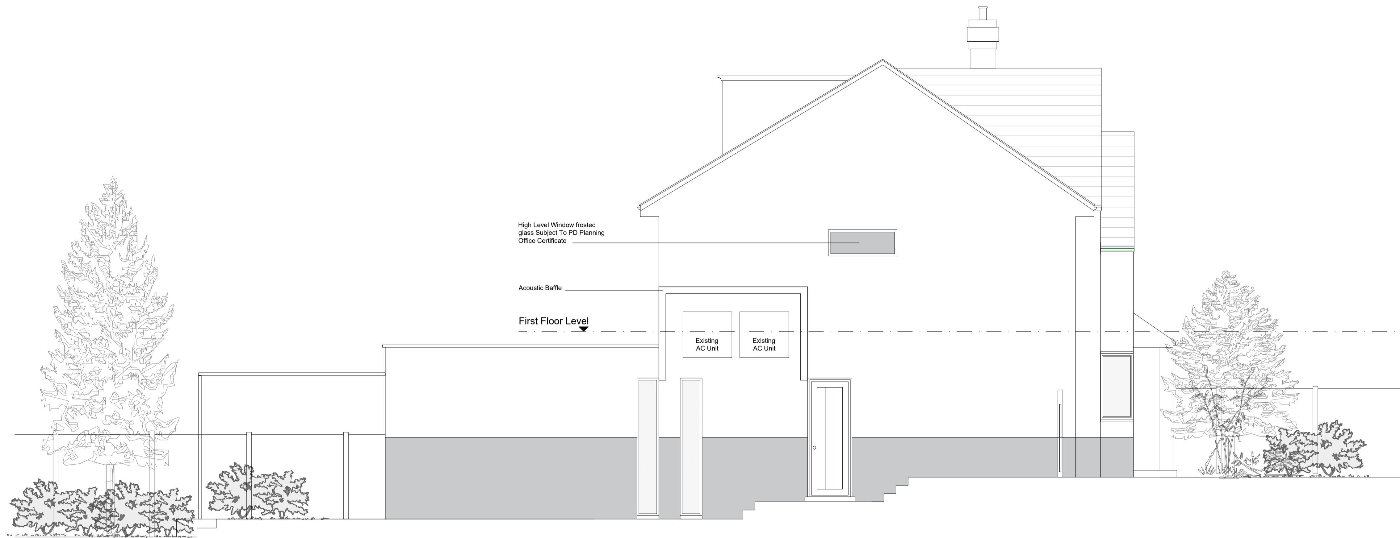
01 South East Side Elevation- PROPOSED scale 1:50
