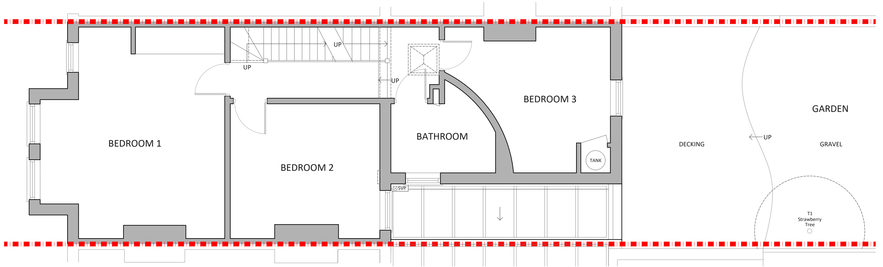
EXISTING FIRST FLOOR PLAN SCALE 1:50
