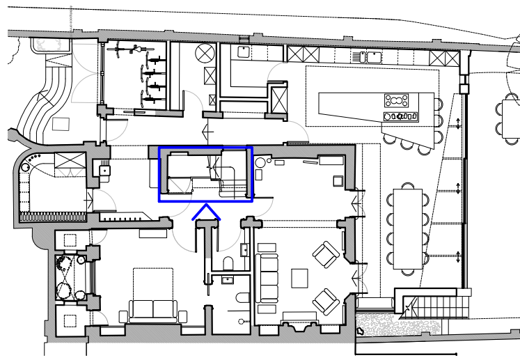
Lower Ground Floor Joinery Location Plan scale 1:200 @ A3
