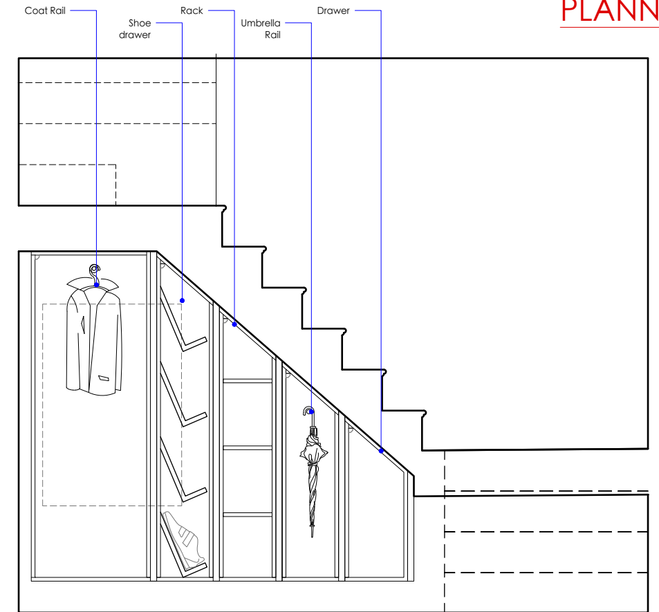
Proposed section scale 1:25 @ A3
