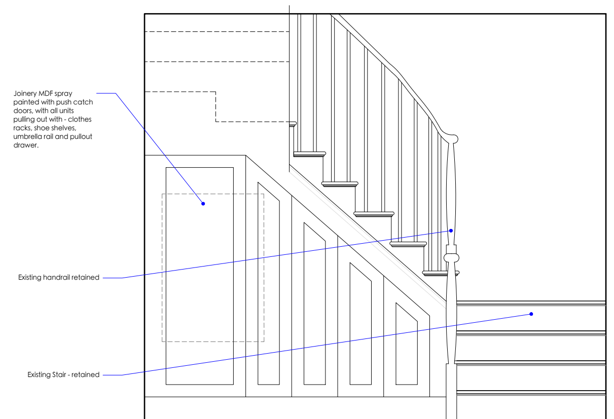
Proposed internal elevation scale 1:25 @ A3
