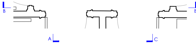
Existing First Floor Landing Plan scale 1:20 at A1
