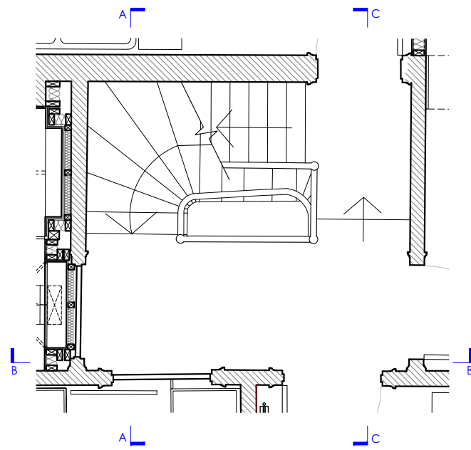
Proposed First Floor Landing Plan scale 1:20 at A1
