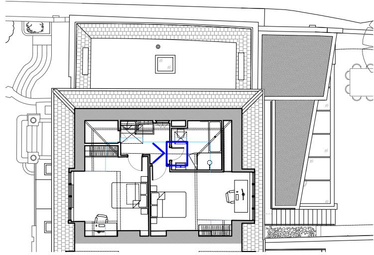
Second Floor Door Location Plan scale 1:200 @ A3
