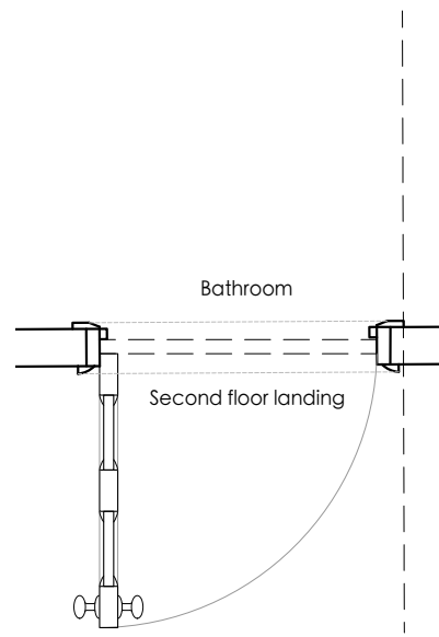
Existing plan scale 1:20 @ A3
