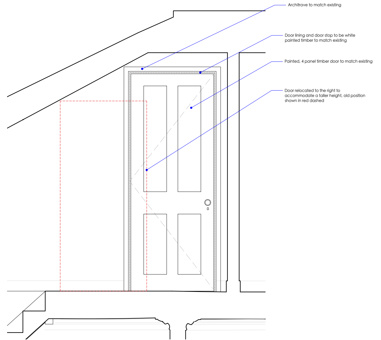
Proposed internal elevation scale 1:20 @ A3
